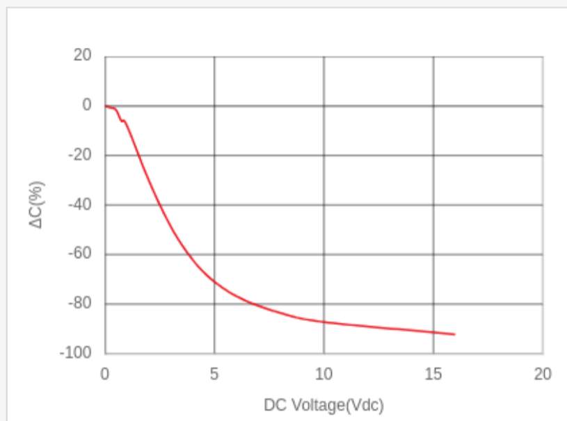
DC Bias Characteristics LCR meter, 1kHz, 1Vrms
