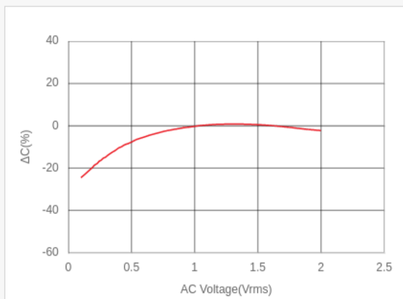
AC Voltage Characteristics LCR meter, 1kHz
