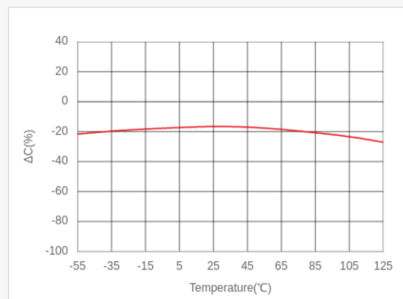
Bias TCC Characteristics LCR meter, 1kHz, 1Vrms, 5Vdc
