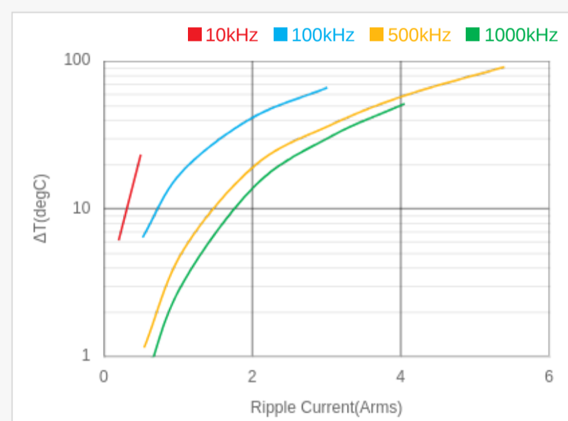
Temperature Rise by Ripple Current
